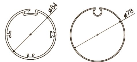
ROLLER TUBE
